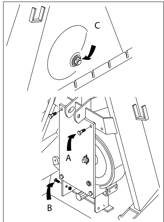
Fig. 19. Removing the winch mechanism
